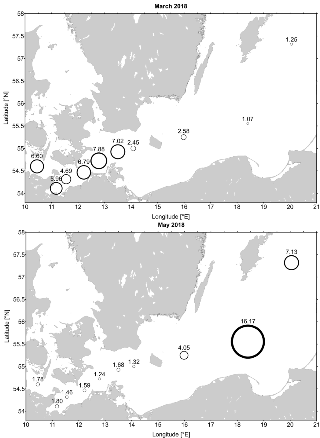
Fig. 21: Horizontal distribution of chlorophyll a concentrations (µg/L) at sampling locations during monitoring cruises in March and May 2018.
