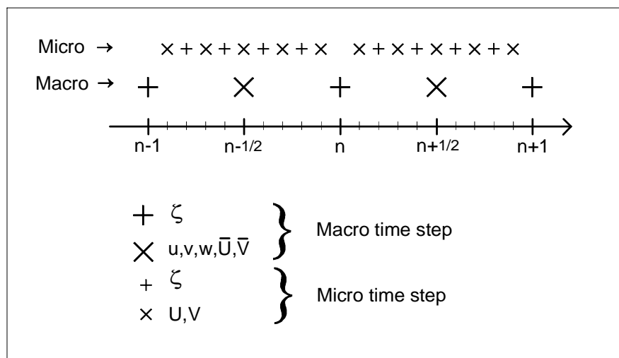
Figure 3.3: Sketch explaining the organisation of the time stepping in GETM. This figure has been taken from Burchard and Bolding [2002].
