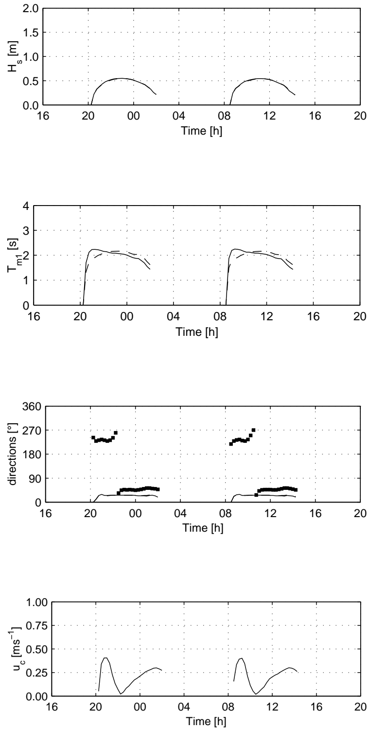
Figure 6.4: Time series of integrated wave parameters and the current velocities for the the wind scenario S1 at the location P2. Line style as in figure (6.3).
