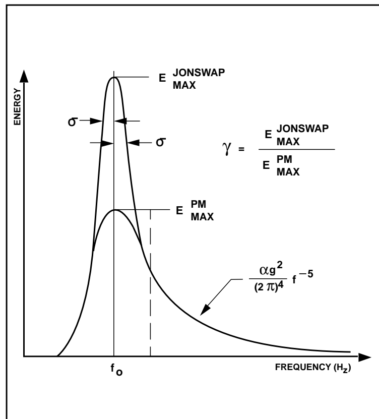
Figure A.1: Comparison of the PM and JONSWAP spectra (Figure adapted from Hasselmann et al., 1973)
