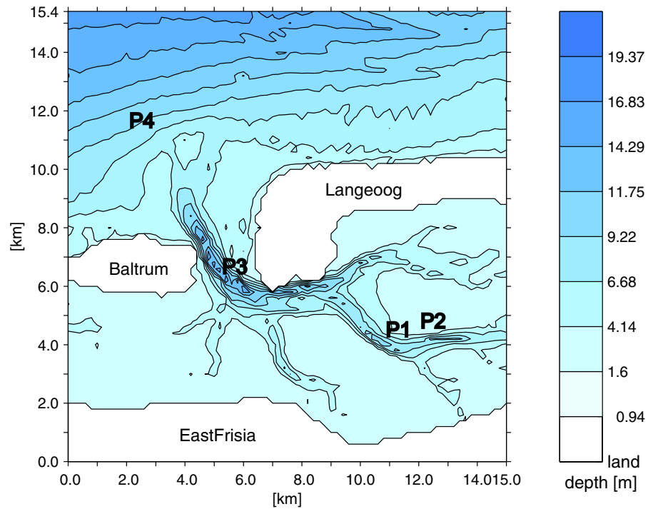
Figure 5.3: The topography of the model area.
