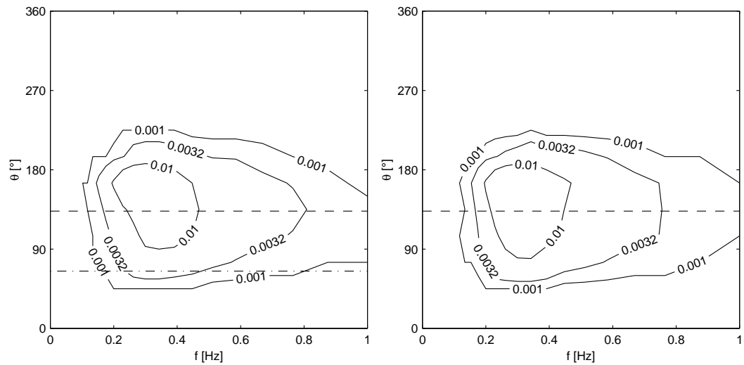
(b) P2 flat, wind scenario S2, two hours after high tide
