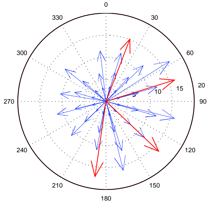
Figure 5.5: Average wind velocities in the direction-speed bins. The velocities chosen for the case studies are presented in red color.
