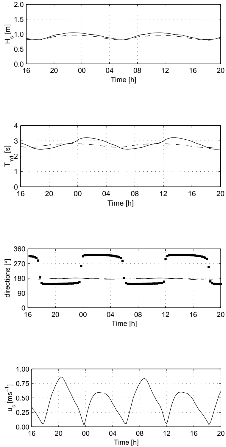
Figure 6.6: Time series of integrated wave parameters and the current velocities for the the wind scenario S4 at the location P3. Line style as in figure (6.3).
