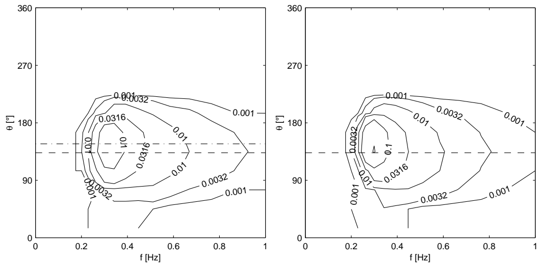
(b) P3 inlet, wind scenario S2, one hour before high tide
