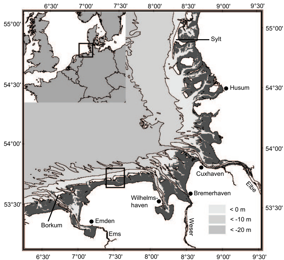
Figure 5.2: Map of the North Sea and the German Bight. The inset depicts the North Sea with the German Bight margined by the square. In the big map of the German Bight the square delimits the model area. The dark shading marks approximately the part of the German Bight that periodically falls dry. (The figure has been adapted from Stanev et al. (2002).)
