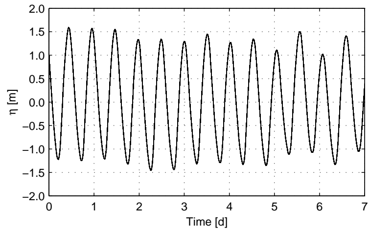
Figure 5.4: Time series of sea level data.
