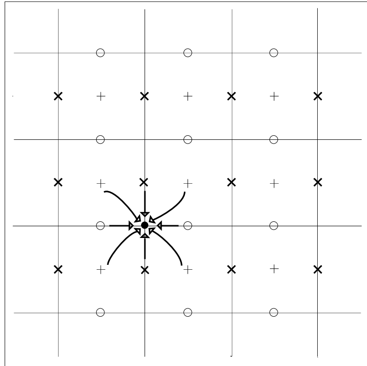
Figure 5.1: Illustration of the interpolation from the Arkawa C-grid of the current model to the non-staggered grid of the wave model. The arrows indicate which values were taken into account.
