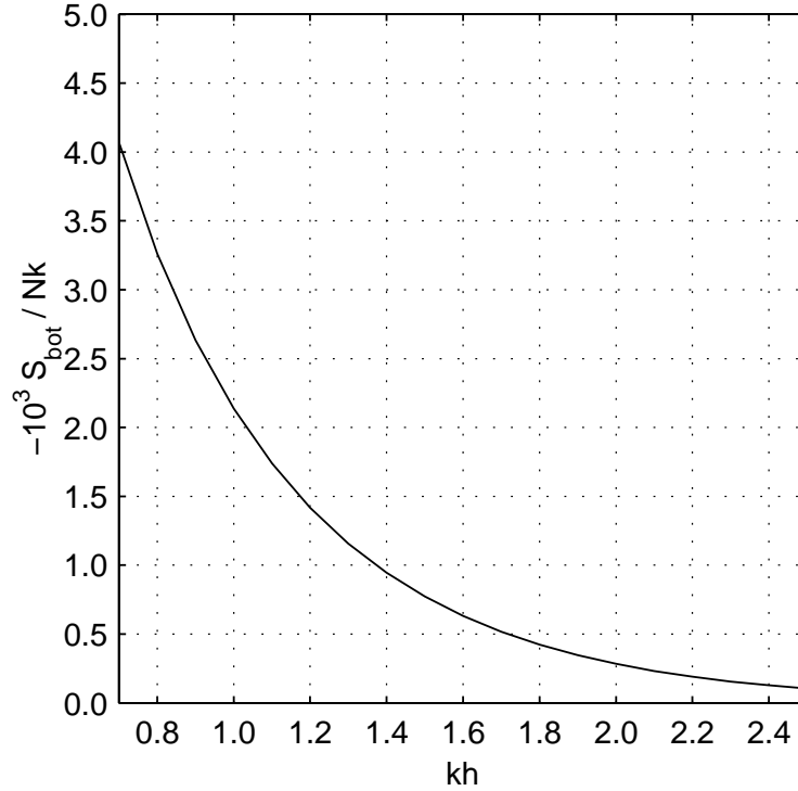
Figure 3.2: The bottom dissipation rate -S_{bot}/N divided by the wavenumber k as a function of nondimensional water depth kh for the interaction coefficient \Gamma = 0.038 \text{ m}^2\text{s}^{-3} (Figure adapted from Komen et al., 1994).
