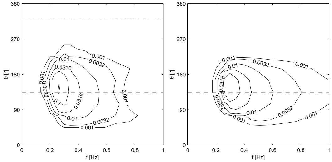
(a) P3 inlet, wind scenario S2, three hours after high tide
