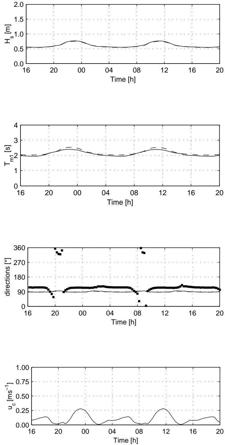
Figure 6.5: Time series of integrated wave parameters and the current velocities for the the wind scenario S3 at the location P1. Line style as in figure (6.3).
