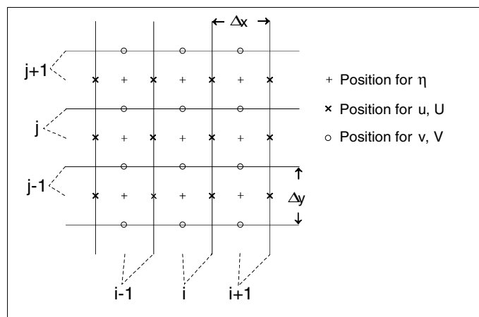
Figure 4.1: The horizontal Arakawa C-grid of GETM (the figure has been adapted from Burchard & Bolding (2002))
