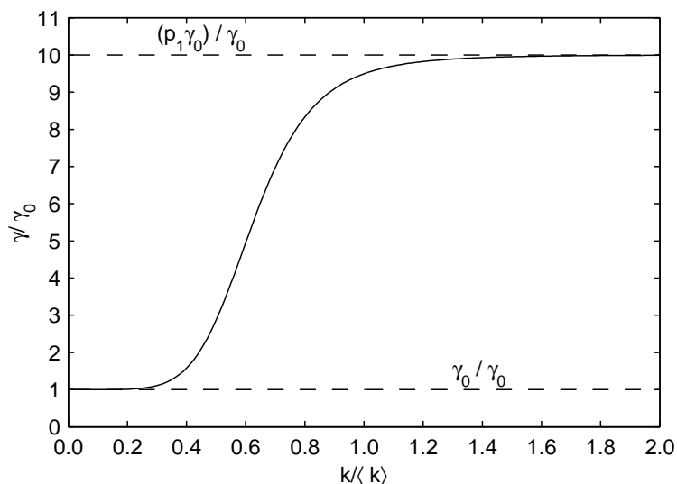
Figure 3.3: The dissipation parameter \gamma of the nonlinear dissipation source function for the values given in the text (Figure adapted from Schneggenburger, 1998).
