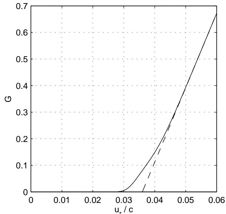
Figure 3.1: Growth rate for a gustiness level of \sigma_{u_*}/u_* = 0.4 . The straight dashed line represents the wave growth in absence of wind gusts (Figure adapted from Komen et al., 1994).
