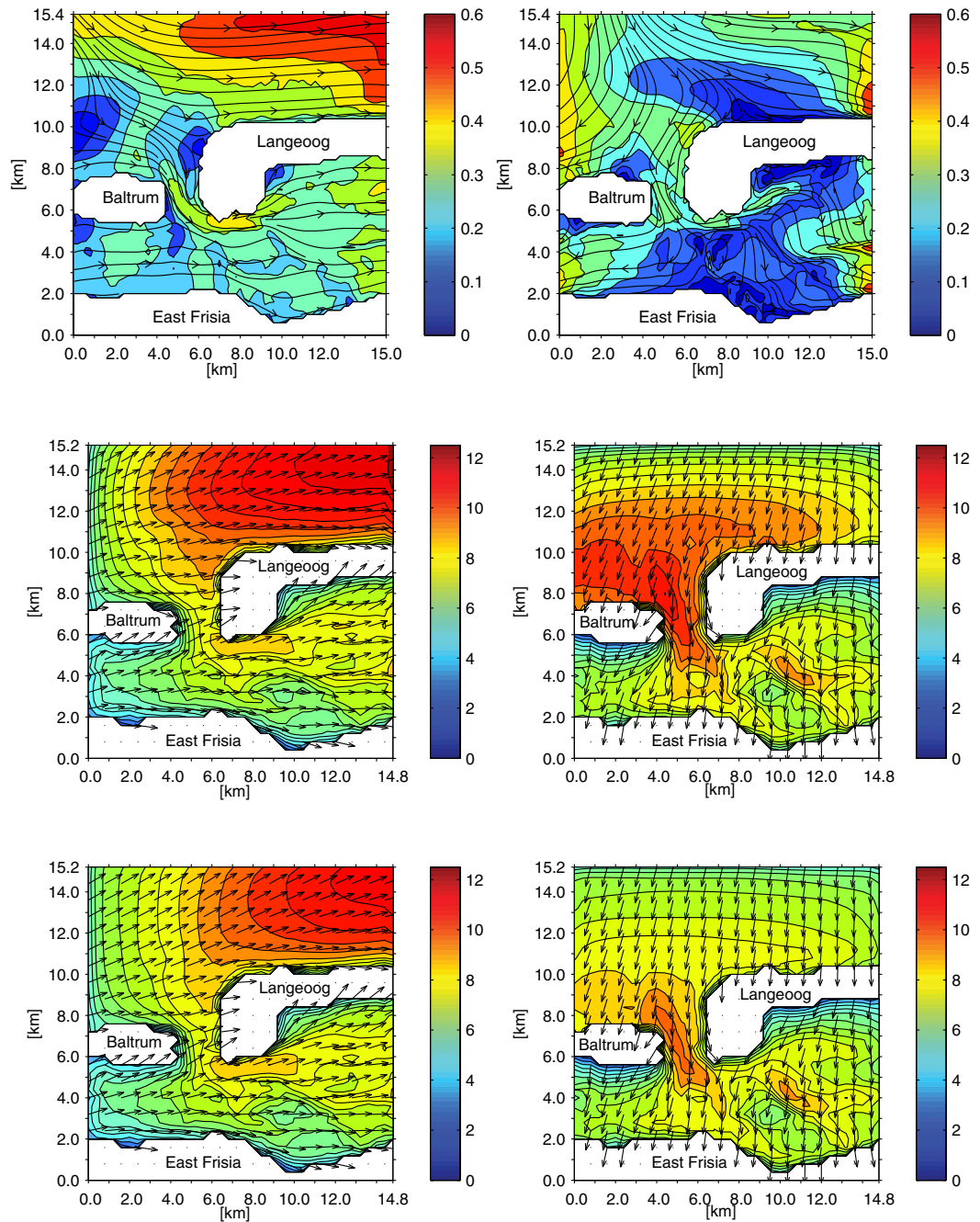
Figure 6.8: Fields of the current velocity and the significant wave height for the stated scenarios
