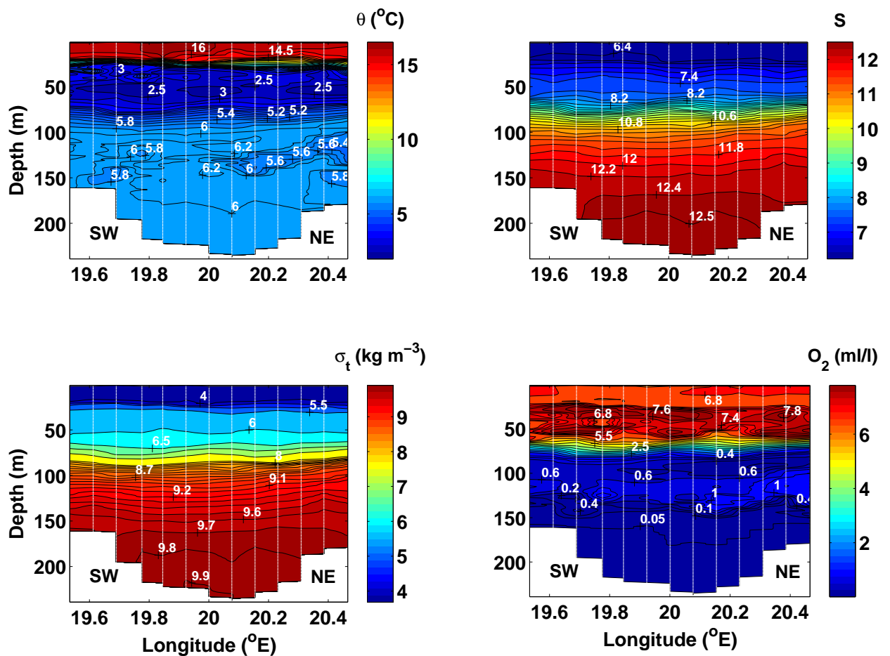
Figure 4.1: Cross-sections through the EGB from NE to SW of potential temperature (upper left), salinity (upper right), density (lower left) and oxygen (lower right panel) on 26 September 2006. The position of the cross-section is marked in Fig. 1.1.
