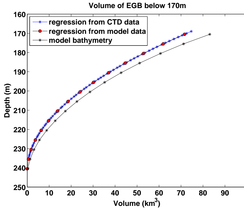
Figure 4.16: Calculated volume of the EGB from CTD data (blue stars) and from model data (red circles). The black line and stars show volume taken from model bathymetry.
