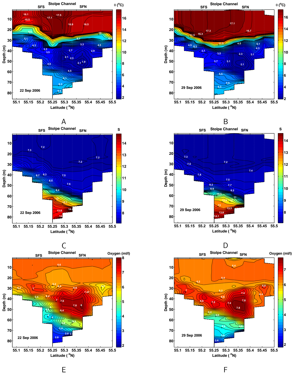
Figure 4.8: The Stolpe Channel: Meridional cross-section at longitude 17.5^{\circ} E of pot. temperature vs. depth (A, B), salinity vs. depth (C, D) and oxygen vs. depth (E, F) on 22 September 2006 (left panels) and 29 September 2006 (right panels). SFN and SFS mark the locations of the ADCPs. The position of the section is marked in Fig. 1.1.
