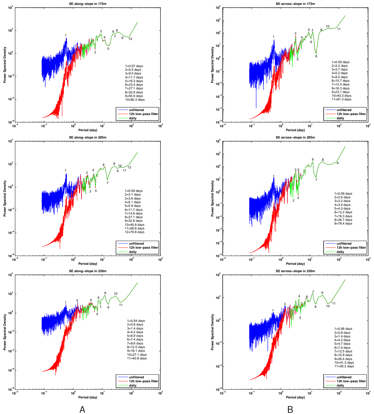
Figure 5.11: Mooring SE: Spectra in 175 m, 205 m and 220 m of the along-slope current component (A) and the across-slope current component (B) for a period from 8 May 2006 to 30 March 2007.
