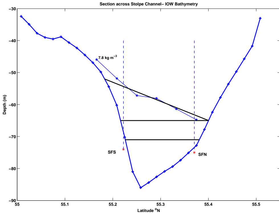
Figure 4.14: Sketch of volume transport calculations through the Stolpe Channel.
