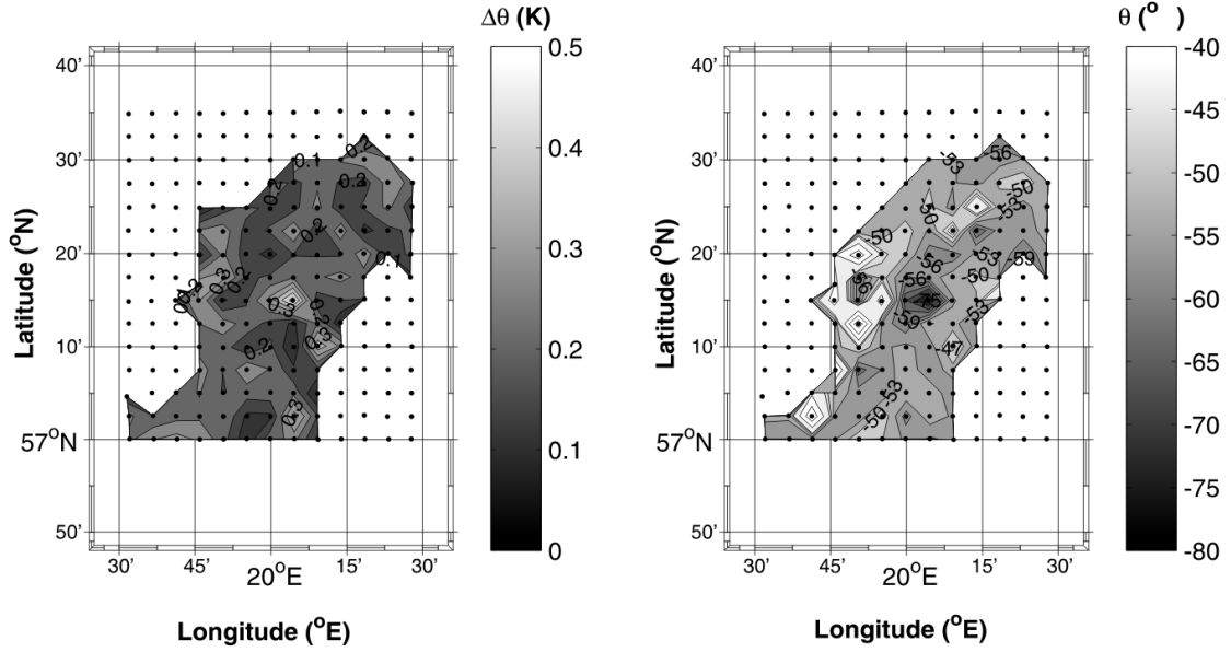
Figure 3.4: a) Difference in potential temperatures ( \Delta\theta ) between the potential density surfaces \sigma_\theta = 9.5 \text{ kg/m}^3 and \sigma_\theta = 9.4 \text{ kg/m}^3 measured during the end of the deep water inflow (M-8). b) The Turner angle on potential density surface \sigma_\theta = 9.5 \text{ kg/m}^3 at the end of the deep water inflow (M-8). Values between -90^\circ and -48.81^\circ (or 1/15 < R_\rho < 1 ) suggest diffusive convective mixing (lighter grey to black).
