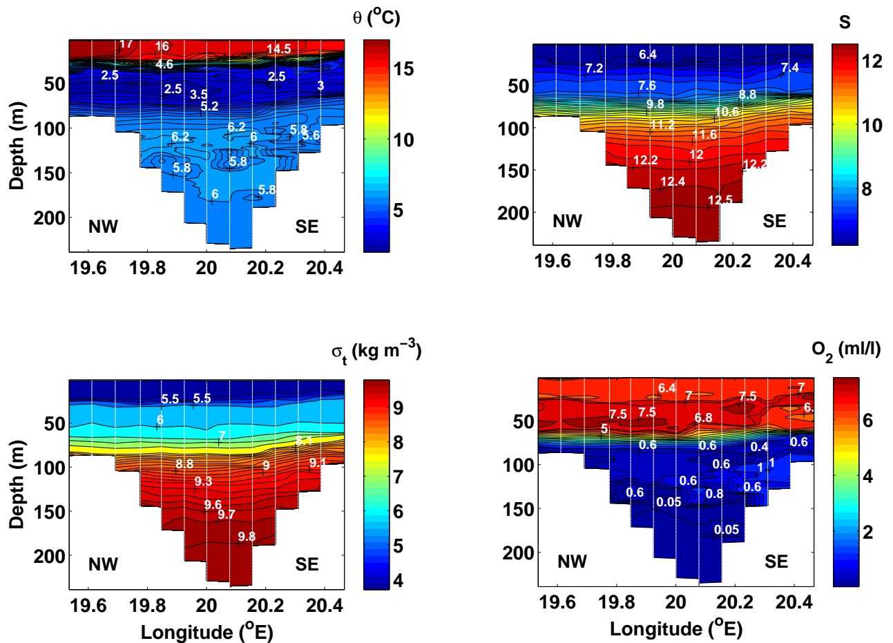
Figure 4.2: Cross-sections through the EGB from NW to SE of potential temperature (upper left), salinity (upper right), density (lower left) and oxygen (lower right panel) on 27 September 2006. The position of the cross-section is marked in Fig. 1.1.
