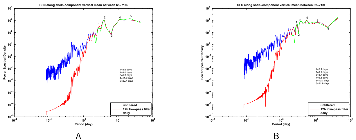
Figure 5.10: The Stolpe Channel: Power spectra of the along-slope vertical mean currents of (A) SFN (between 65-71 m) and (B) SFS (between 52-71 m) for a period from 23 September to 19 December 2006.
