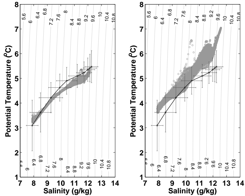
Figure 3.2: \theta/S plots of hydrographic stations M-7 (grey circles, left panel) and M-8 (grey circles, right panel) below 60 m. M-7 was conducted between 29 August - 04 September 1997, M-8 between 19 - 24 April 1998. The black line is the 30 yr mean with standard deviations of potential temperature ( \theta ) and salinity ( S ) of BMP271. BMP271 and station grid of M-7/M-8 are shown in Fig. 1.2.
