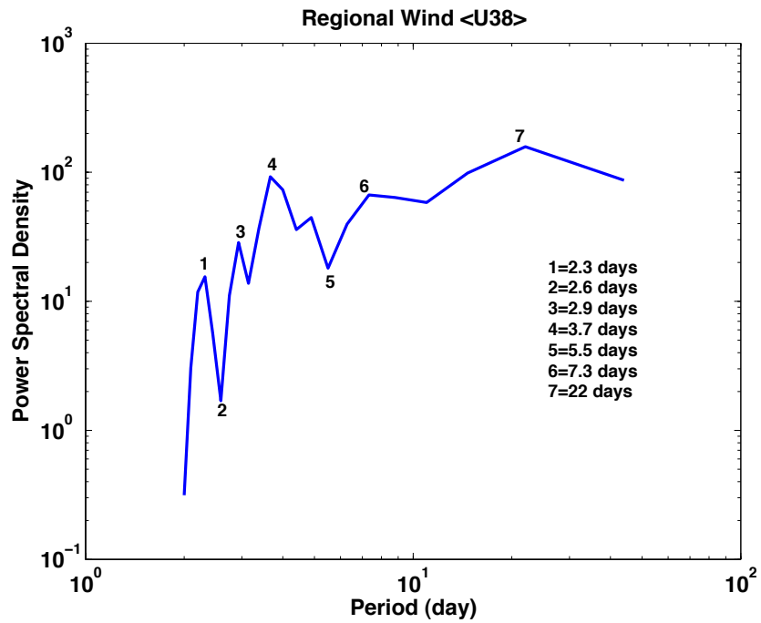
Figure 5.9: Power spectrum of averaged wind \langle U \rangle_{38} .
