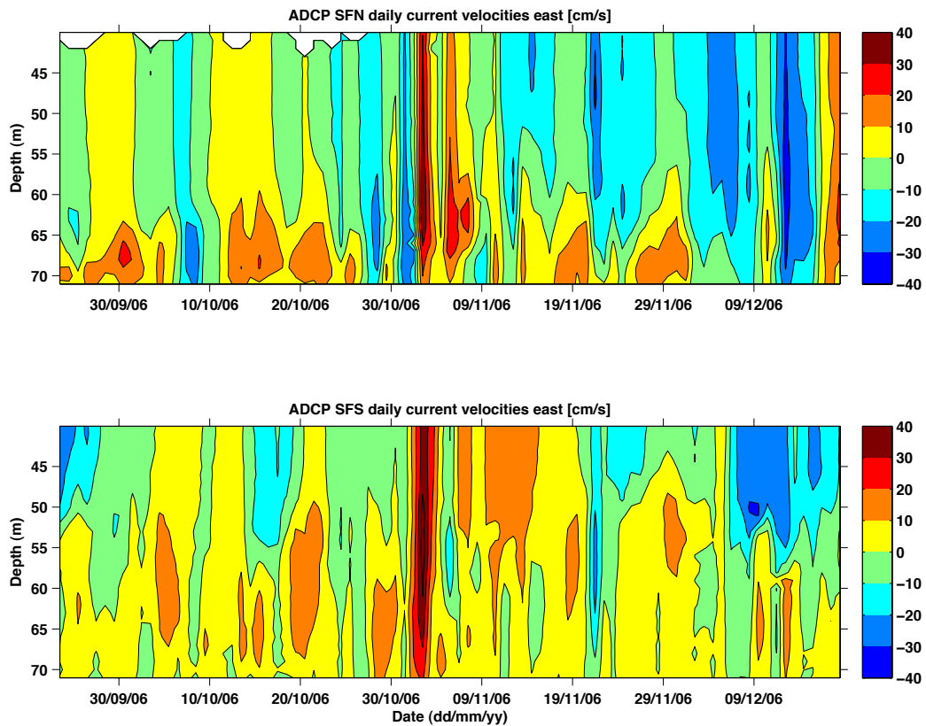
Figure 4.12: Daily zonal current velocities of ADCP moorings SFN and SFS.
