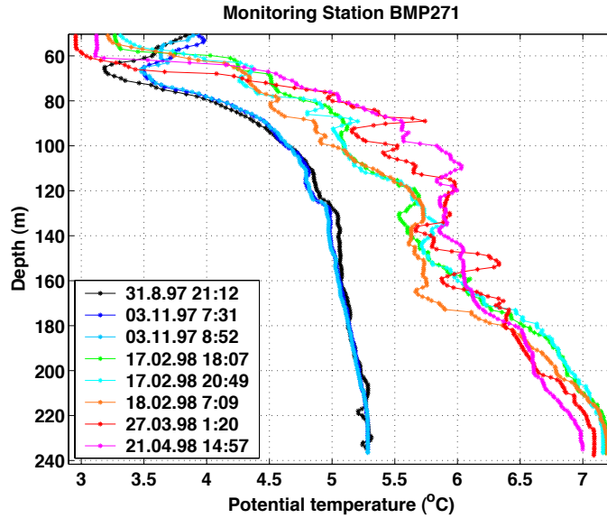
Figure 3.7: Potential temperature vs. depth of the monitoring station BMP271 below 50 m to the bottom, see Fig. 1.2. Sampling time given as dd.mm.yy HH:MM UTC.
