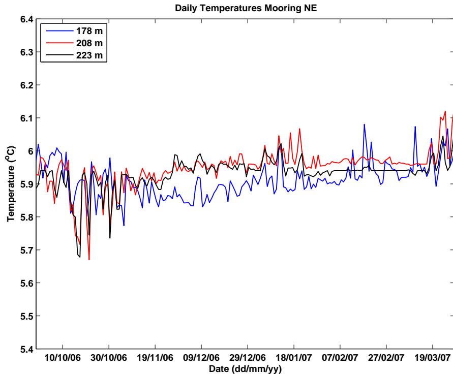
Figure 4.5: Temperatures in 178, 208 and 223 m depth of mooring NE. Note the different time scale compared to other two moorings.
