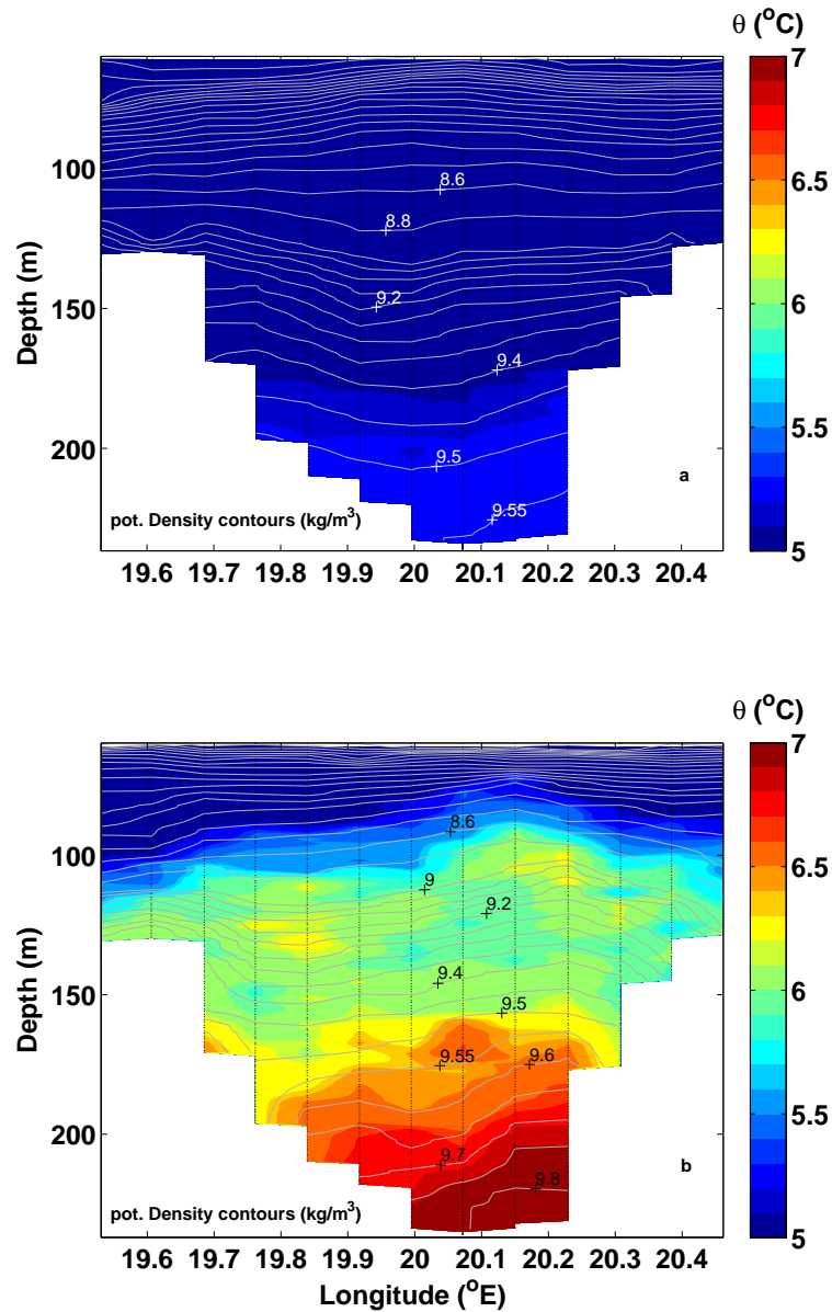
Figure 3.5: Horizontal section of potential temperature vs. depth and density contours of M-7 (a) and M-8 (b) at latitude 57.24°N. Its position is marked as a horizontal line in Fig. 1.2.
