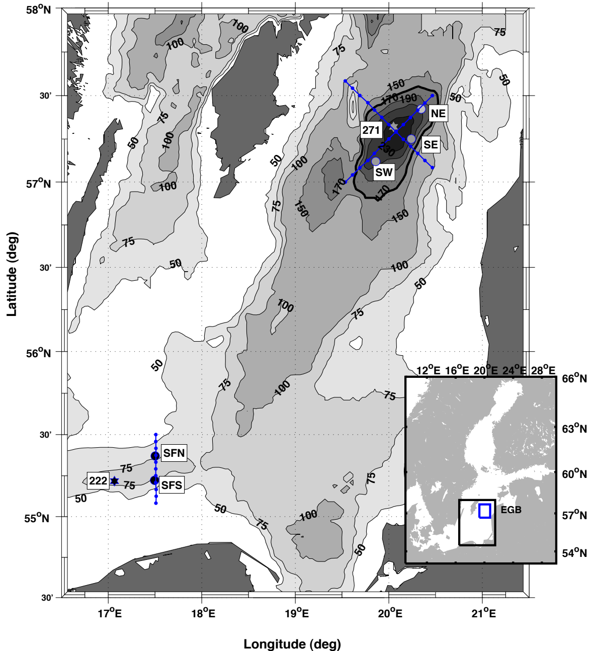
Figure 1.1: Bathymetric map of research area (inserted Eastern Gotland Basin, EGB, blue Square) in the Baltic Sea. SFN and SFS are ADCP mooring positions within the Stolpe Channel (SF); Dots mark mooring positions SE, NE and SW within the EGB. Stars mark the positions of central HELCOM-monitoring stations 222 (SF) and 271 (EGB). Dotted blue lines indicate CTD transects across the Stolpe Channel and through the EGB.
