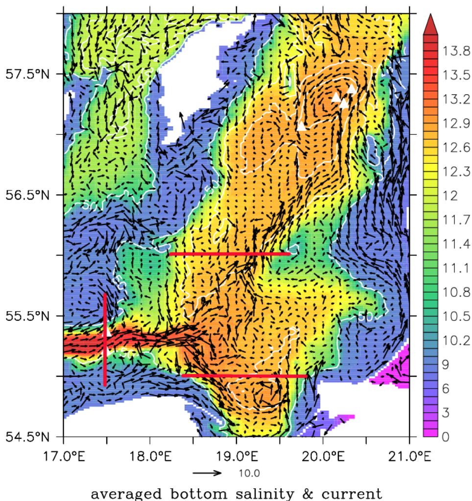
Figure 4.18: Propagation of the deep water in the bottom boundary layer (black arrows) and mean salinity distribution for the Baltic Proper, simulated with MOM4. T, S, depth and currents were extracted as 5-day means for 3 selected transects (red lines). White triangles represent mooring positions.
