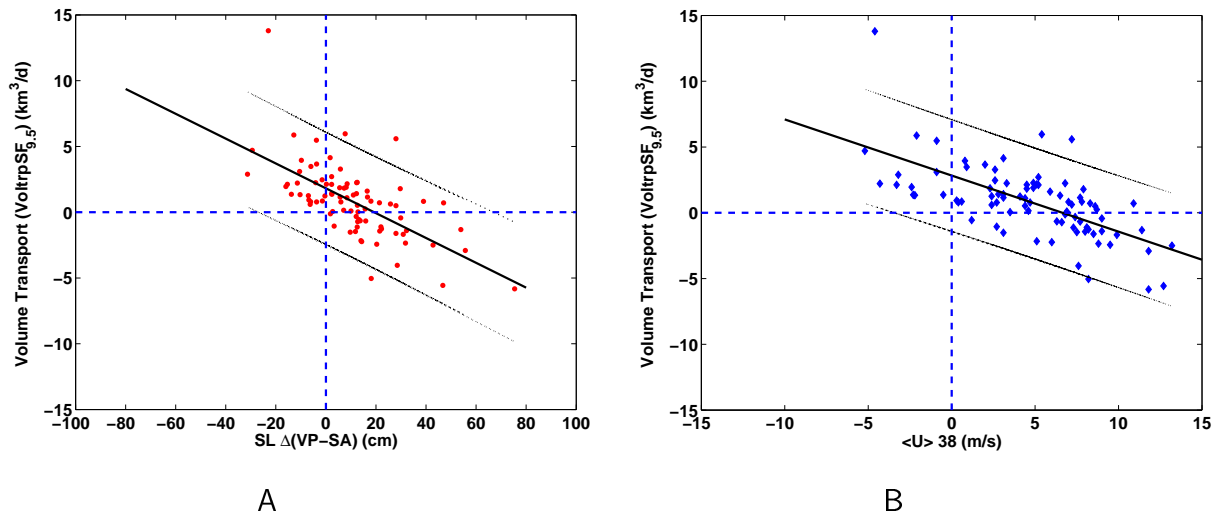
Figure 4.32: Regression SL \Delta (Ventspils-Sassnitz) with pos./neg. volume transport below 9.5 \text{ kg/m}^3 Stolpe Channel ( \text{VoltrpSF}_{9.5} ) (A); and wind \langle U \rangle_{38} (Arkona-Hoburg) with pos./neg. volume transport below 9.5 \text{ kg/m}^3 Stolpe Channel ( \text{VoltrpSF}_{9.5} ) (B). The two fine lines correspond to the 95% confidence interval of the regression line (thick line).
