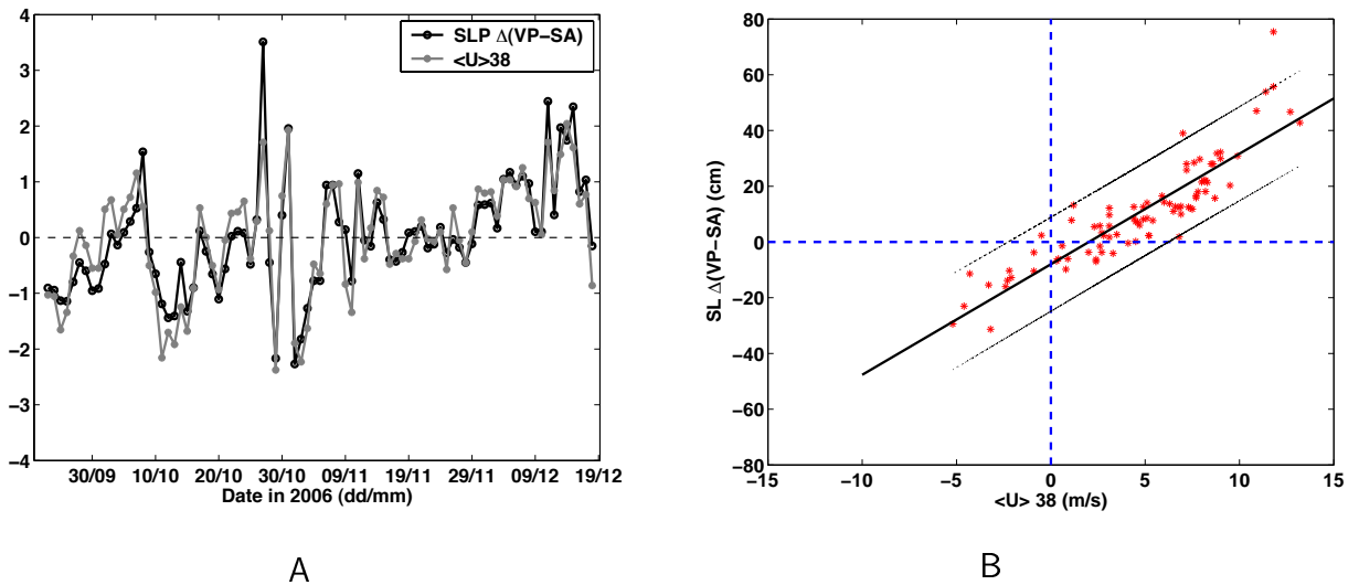
Figure 4.29: A: Standardised time series of \langle U \rangle_{38} (grey) and SL \Delta(VP-SA) (black). B: Regression wind \langle U \rangle_{38} (Arkona-Hoburg) with SL \Delta(VP-SA) . The two fine lines correspond to the 95% confidence interval of the regression line (thick line).
