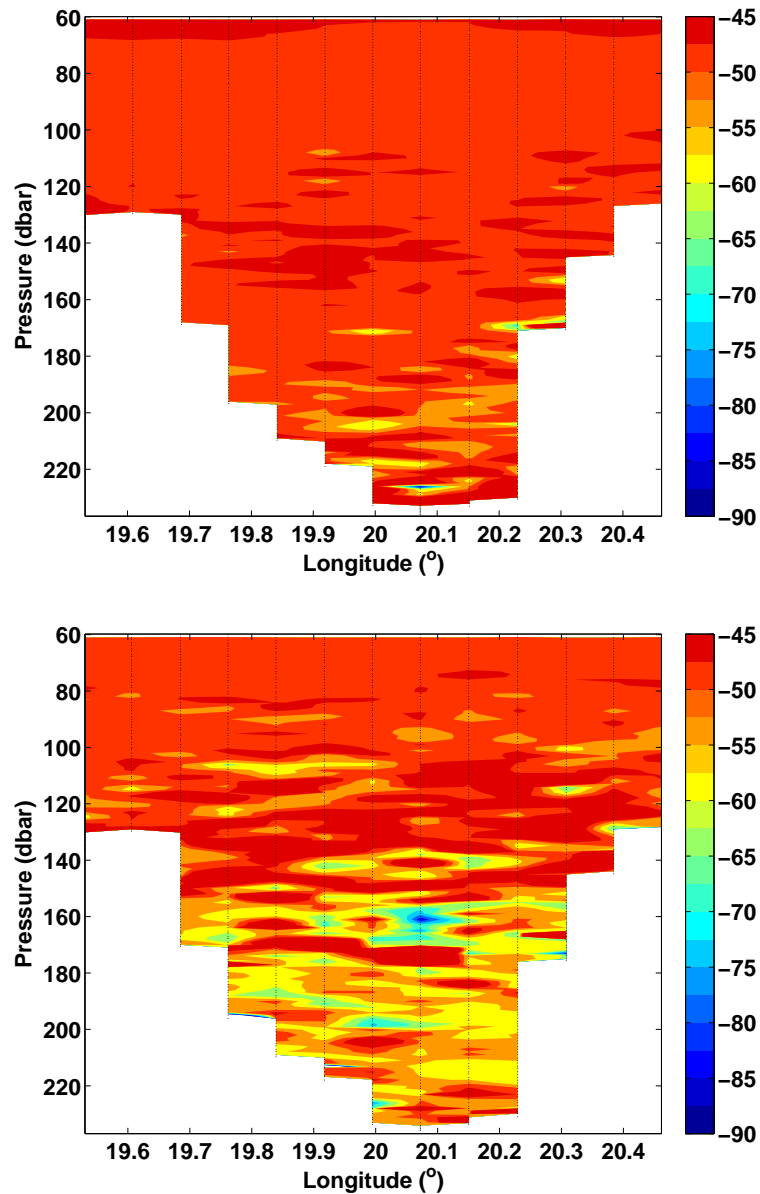
Figure 3.6: Transect as in Fig. 3.5, but for Turner angles in the diffusive convective regime, with Tu < -48.81^\circ (dark red) or R_\rho > 1/15 as the lower bound of diffusive convection.
