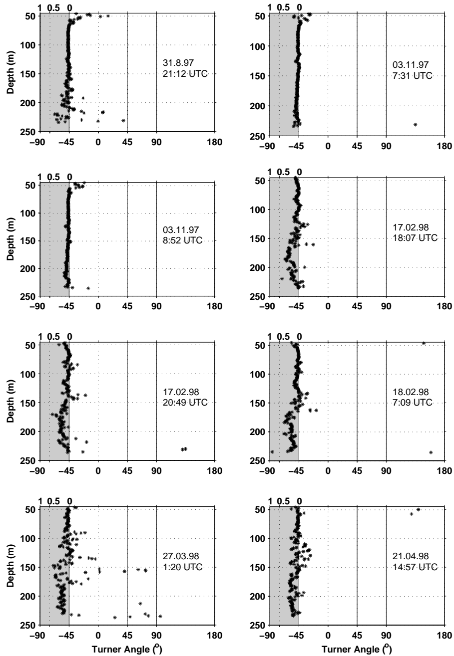
Figure 3.8: Turner angles vs. depth profiles of monitoring station BMP271 between 31 August 1997 and 21 April 1998. Grey area indicates diffusive convective regime ( -90^\circ < Tu < -45^\circ ). Top x-axis indicates associated density ratios for R_\rho = 0, 0.5, \text{ and } 1 . Sampling time given as dd.mm.yy HH:MM UTC.
