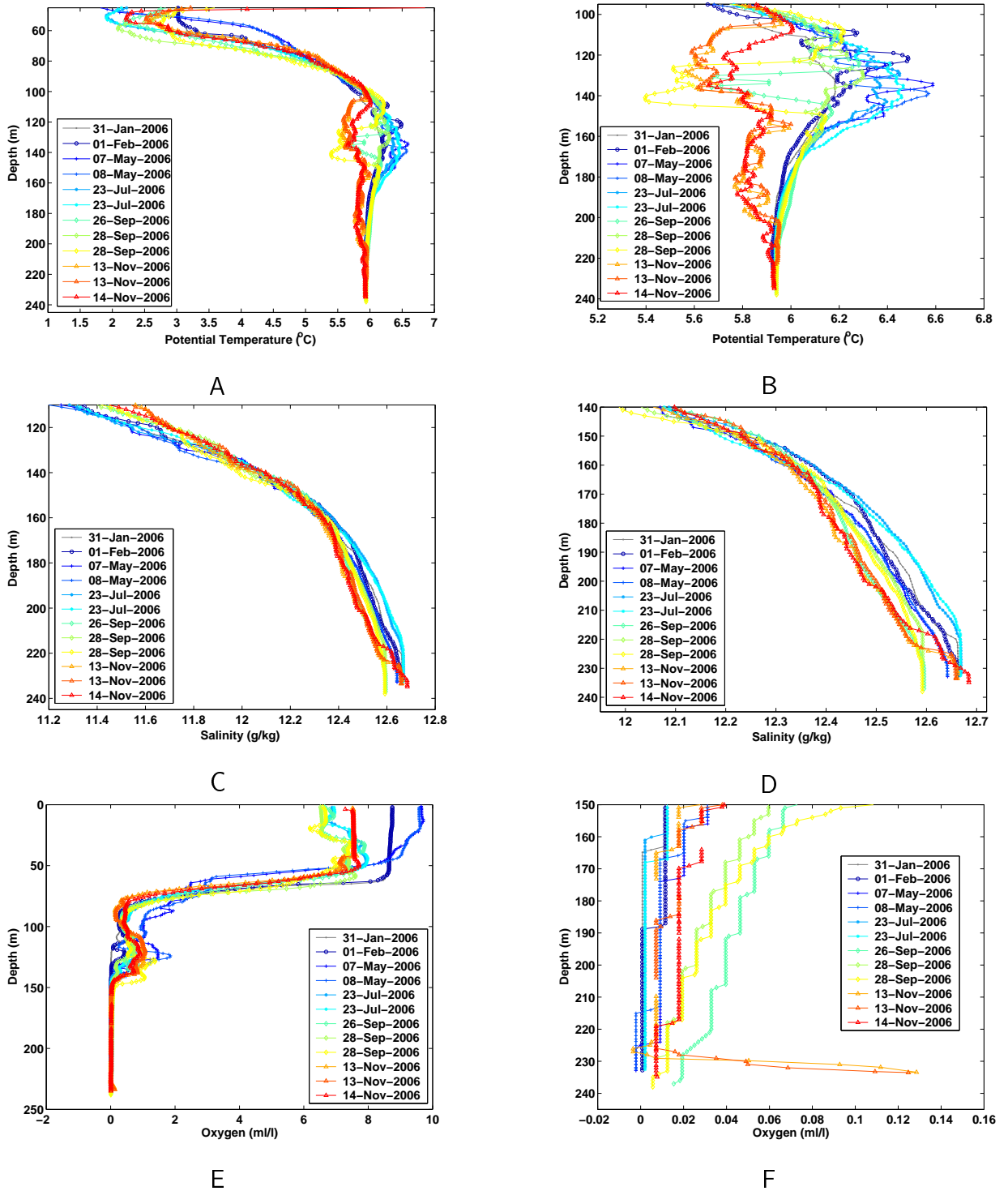
Figure 4.3: Potential temperature (A and B), Salinity (C and D) and Oxygen (E and F) depth profiles at central monitoring station of EGB (BMP271) in January, February, May, July, September and November 2006. The position is marked in Fig. 1.2.
