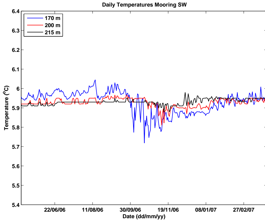
Figure 4.6: Temperatures in 170, 200 and 215 m depth of mooring SW.
