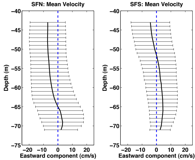
Figure 4.13: Temporal mean (23 September to 19 December 2006) of the current velocity east vs. depth with error bars for SFN (left panel) and SFS (right panel).
