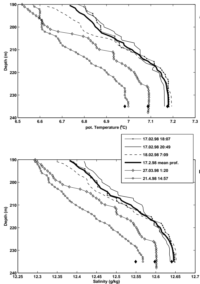
Figure 3.10: (a) Potential Temperature vs. depth, (b) salinity vs. depth of BMP271 on 17-18 February 1998, 17 February 1998 (mean profile), 27 March 1998 and 21 April 1998. Sampling time given as dd.mm.yy HH:MM UTC. Diamonds represent the corresponding potential temperature and salinity averages of the basin's volume between 225-235 m.
