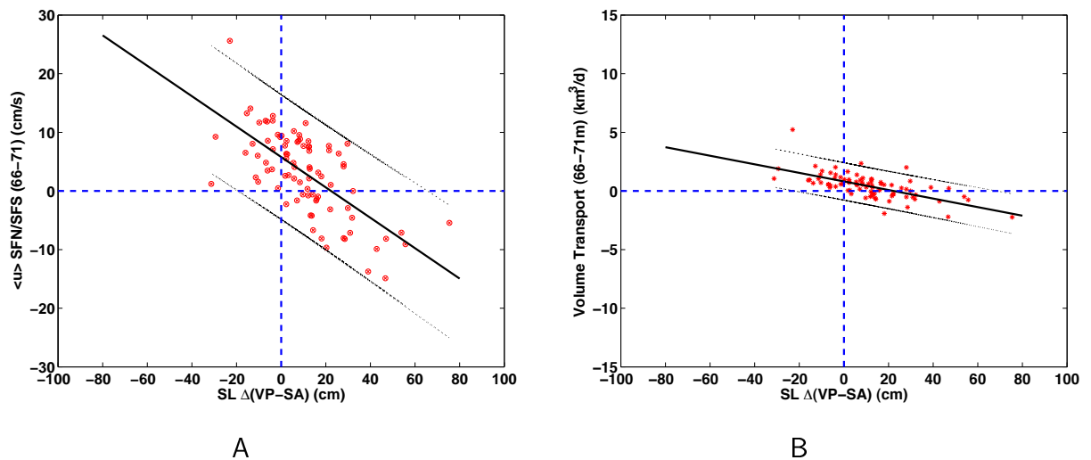
Figure 4.31: Regression SL \Delta (Ventspils-Sassnitz) with measured depth averaged zonal velocity from ADCPs (A). SL \Delta (Ventspils-Sassnitz) with volume transport (66 – 71 m) (VoltrpSF ADCP66-71 ) Stolpe Channel (B). The two fine lines correspond to the 95% confidence interval of the regression line (thick line).
