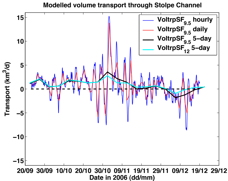
Figure 4.26: Deep volume transports across the Stolpe Channel from model data. Hourly (blue) and daily transport values (red) were derived from densities higher 9.5 \text{ kg/m}^3 , 5-day transports (cyan) from salinities higher 12\text{g/kg} .
