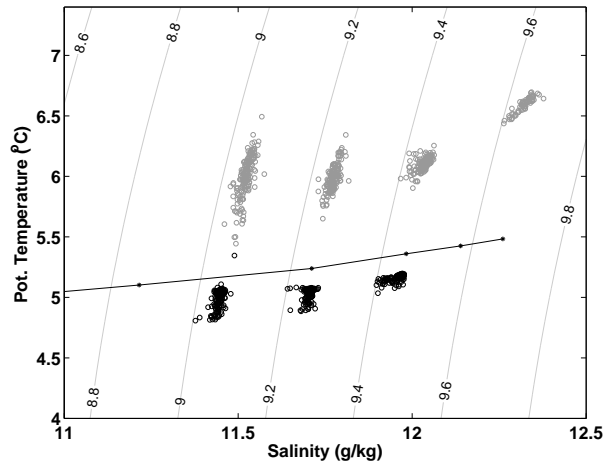
Figure 3.3: \theta/S plots of survey M-7 (black) and M-8 (grey) on potential density surfaces ( \sigma_\theta ) of 9.0 \leq \sigma_\theta < 9.1 \text{ kg/m}^3 , 9.2 \leq \sigma_\theta < 9.3 \text{ kg/m}^3 , 9.4 \leq \sigma_\theta < 9.5 \text{ kg/m}^3 , 9.6 \leq \sigma_\theta < 9.7 \text{ kg/m}^3 , before and during the terminating deep water inflow; thin lateral line corresponds to 30 year averages of station BMP271.
