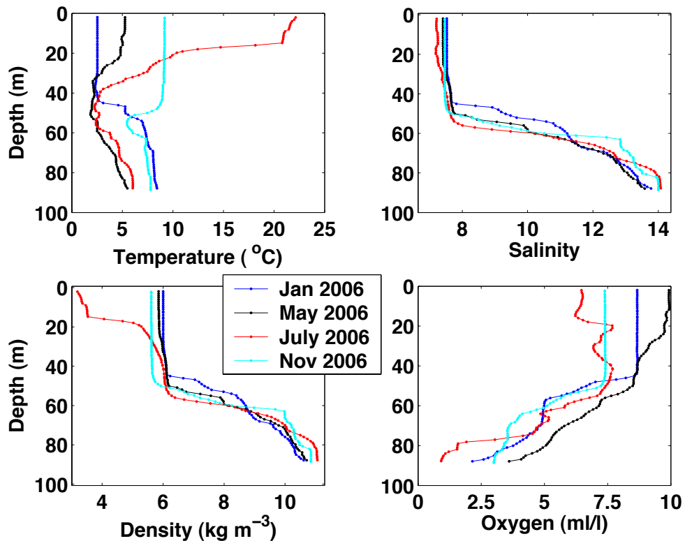
Figure 4.7: Depth profiles of temperature, salinity, density and oxygen of the central monitoring station of the Stolpe Channel (BMP222) for January, May, July and November 2006.
