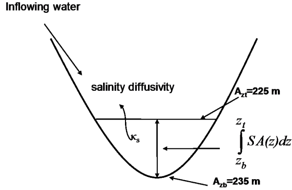
Figure 3.9: Sketch of salinity/ heat budget calculations in the EGB for profiles in shown Fig. 3.10.
