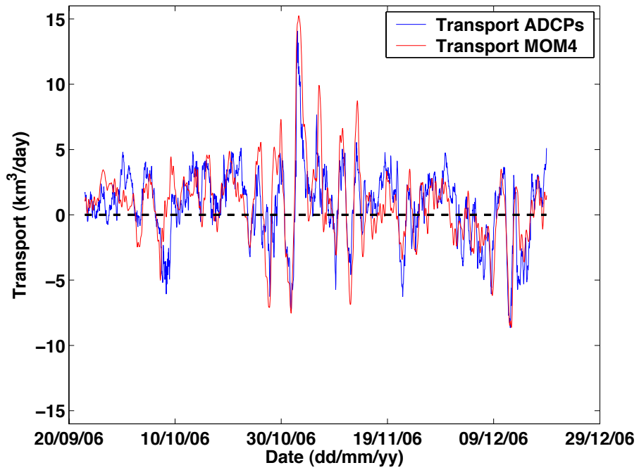
Figure 4.15: Comparison of hourly volume transports through the Stolpe Channel calculated from ADCP measurements with MOM model.
