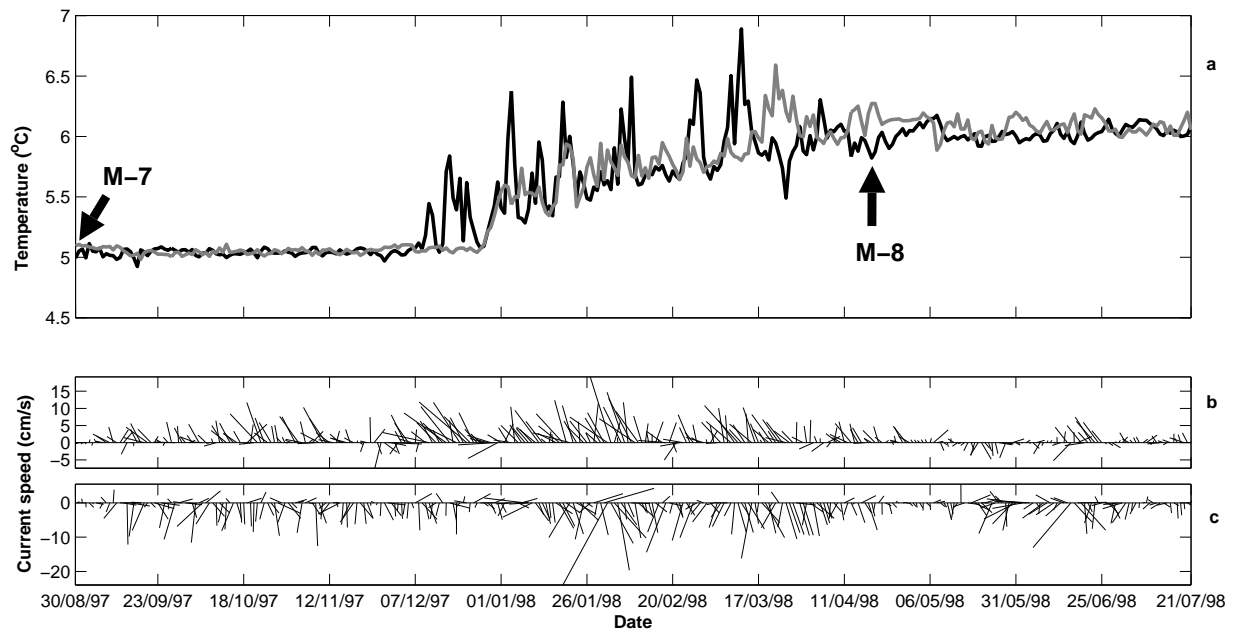
Figure 3.1: Daily temperature and current series of Aanderaa current meters deployed at 170 m depth at positions shown in Fig. 1.2 and statistics compiled in Table 3.1: a) Daily temperature records ( ^{\circ} ) of the NE (black) and SW moorings (grey). Two arrows mark the CTD surveys M-7 (before) and M-8 (during the end of the inflow). Note that the warm deep water inflow reached the NE mooring around the 27 November 1997, but the SW position 30 days later. b) Stick plot of daily current speed (cm/s) of mooring NE and c) stick plot of mooring SW; note the different vertical scales of b) and c). Date displayed as dd/mm/yy.
