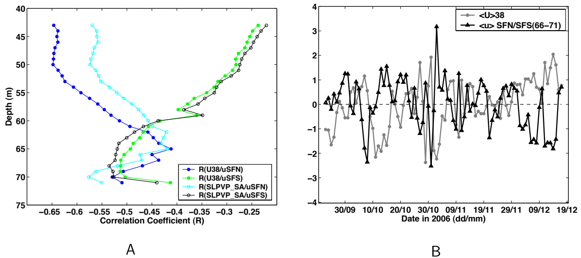
Figure 4.30: A: Correlation coefficients of \langle U \rangle_{38} with u SFN (blue)/ u SFS (green) and SL \Delta (Ventspils-Sassnitz) with u SFN (cyan)/ u SFS (black) in 1 m steps between 43-71 m. B: Standardised time series of \langle U \rangle_{38} (grey) and depth averaged mean current of SFN and SFS (66-71 m, black).
