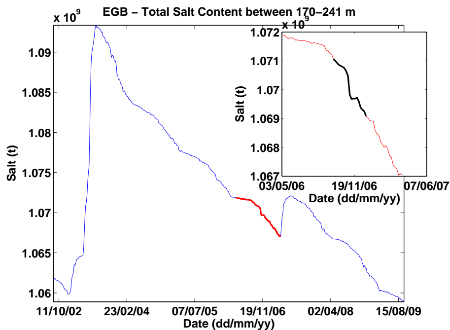
Figure 4.17: Total salt content of the deep EGB greater than 170 m in a volume of 83 km 3 .
