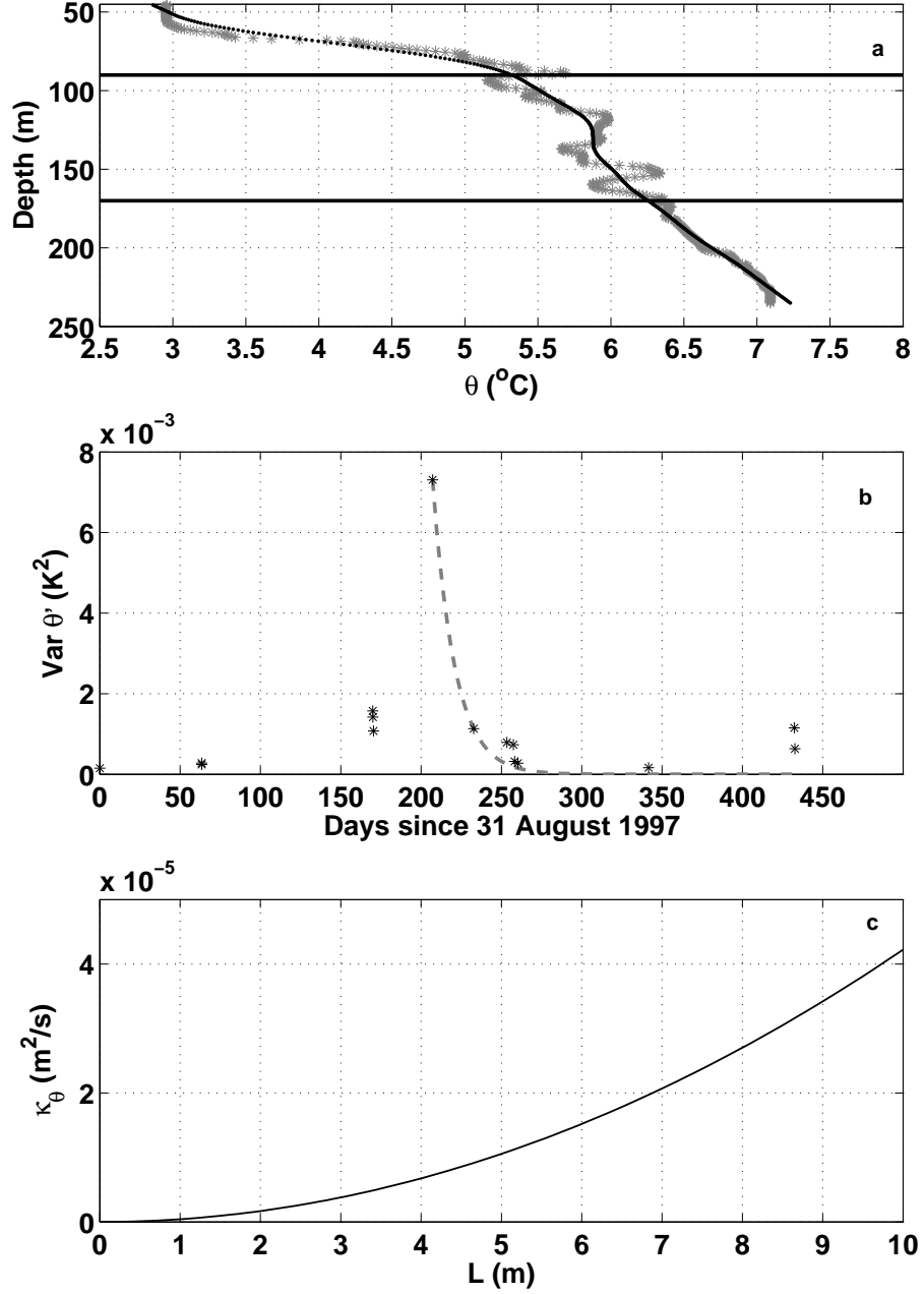
Figure 3.11: (a) Potential temperature profile from 27 March 1998, filtered with a cut-off length of 3 m (grey stars) and 50 m (black dots). Horizontal lines indicate the intrusion layer (90-170 m) used for the analysis; (b) time series of \langle \theta'^2 \rangle (stars) for all available temperature profiles between 31 August 1997 and 7 November 1998, and exponential fit (dashed line); (c) vertical intrusion scale, L , vs. diffusivity of heat, \kappa_\theta .
