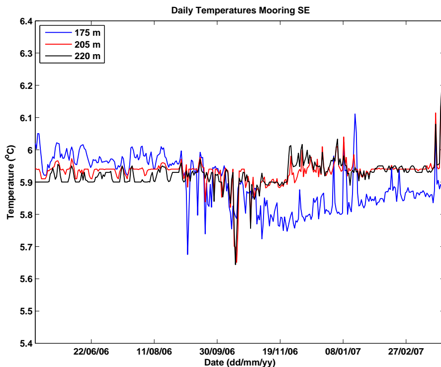
Figure 4.4: Temperatures in 175, 205 and 220 m depth of mooring SE.
