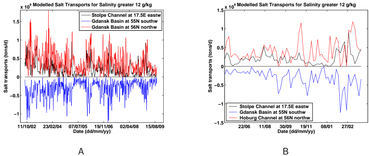
Figure 4.20: Modelled salt transports through three sections in the Baltic proper, Stolpe Channel at 17.5°E, Gdansk Basin at 55°N and Hoburg Channel at 56°N, positions are marked in Fig. 4.18. A: time period 2002 - 2009, B: time period May 2006 - March 2007. Note, scales between plots slightly differ.
