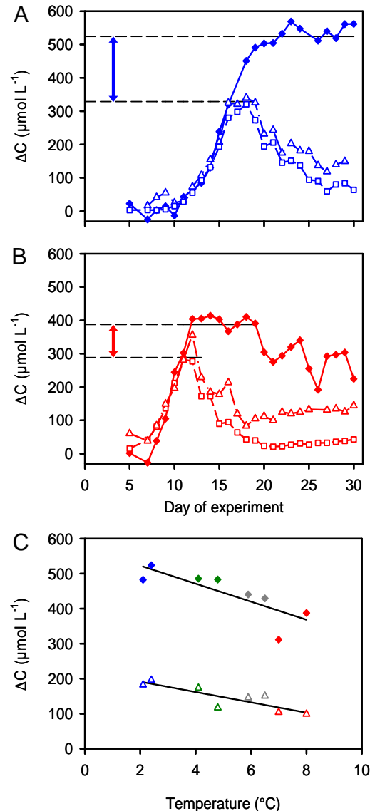
Fig. 2. Temperature sensitivity of inorganic carbon consumption, organic carbon build-up and loss. (A and B) Temporal development of the net draw-down of DIC ( \Delta\text{DIC} ; \blacklozenge /solid line), the net build-up of POC ( \Delta\text{POC} ; \square /dashed line), and the net build-up of TOC ( \Delta\text{TOC} = \Delta\text{POC} + \Delta\text{DOC} ; \triangle /dashed-dotted line) at in situ temperature T+0 (A, blue) and at elevated temperature T+6 (B, red) (data from 1 replicate mesocosm of each treatment). The 2 horizontal lines in each panel indicate the magnitude of the maximum net consumption of DIC ( \Delta\text{DIC}_{\text{max}} , upper line) and the maximum net build-up of TOC ( \Delta\text{TOC}_{\text{max}} , lower line); the arrow indicates the magnitude of the net loss of organic carbon from the water column ( \Delta\text{C}_{\text{loss}} ) at the time of maximum organic carbon accumulation. (C) \Delta\text{DIC}_{\text{max}} ( \blacklozenge ) and \Delta\text{C}_{\text{loss}} ( \triangle ) as a function of temperature. Color code is as in Fig. 1. Solid lines denote linear regressions ( n = 8 ; \Delta\text{DIC}_{\text{max}} : R^2 = 0.66 , P = 0.014 ; \Delta\text{C}_{\text{loss}} : R^2 = 0.74 , P = 0.006 ).
